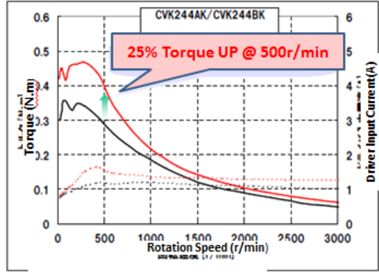
2 Phase Bipolar □42mm
