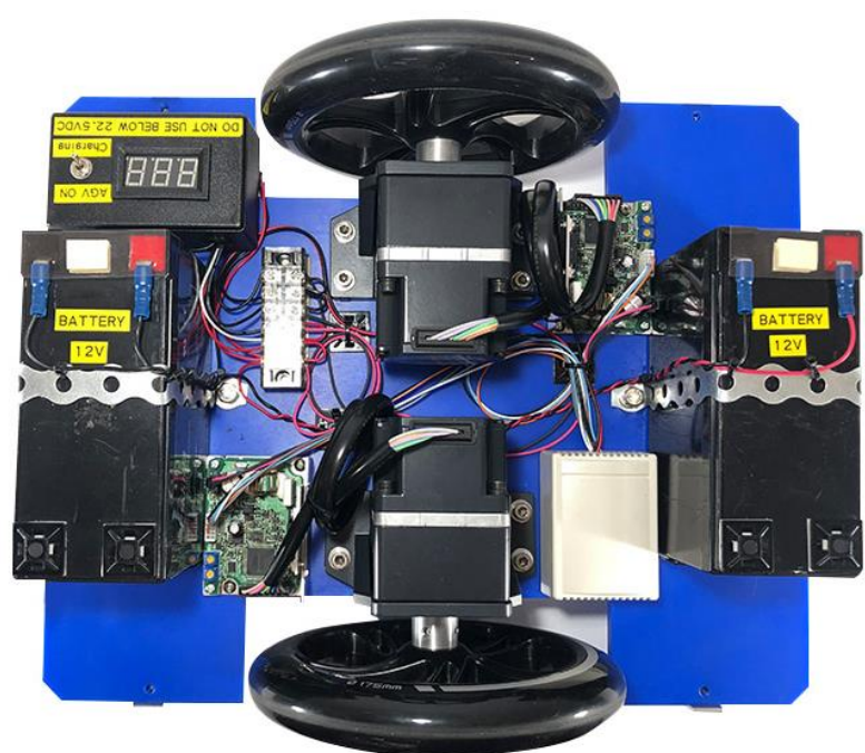
Automated Guided Vehicle Demonstration
